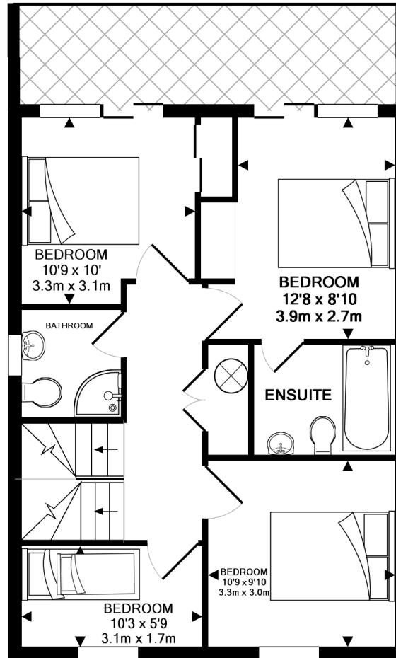
1ST FLOOR APPROX. FLOOR AREA 630 SQ.FT. (58.5 SQ.M.)
